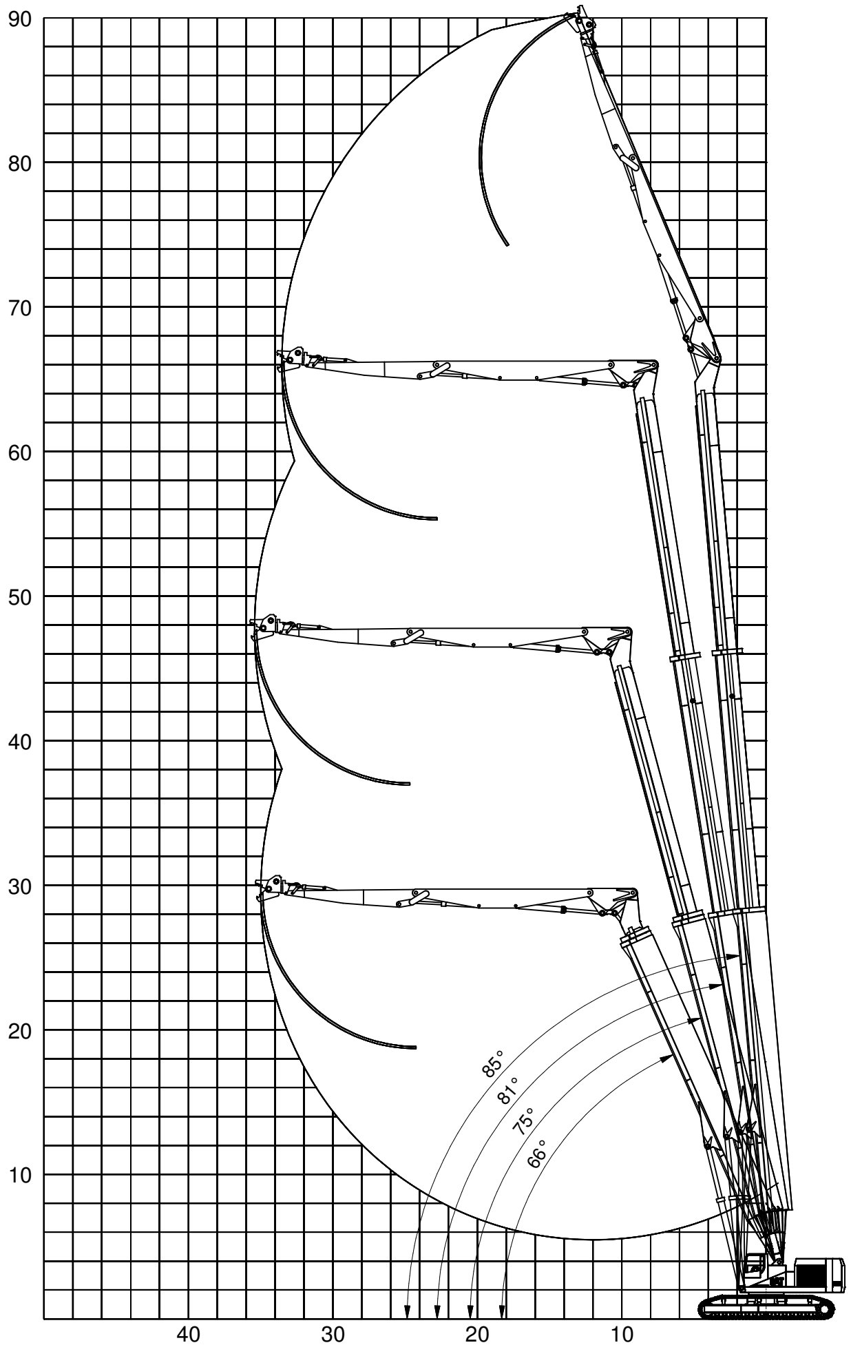
Working-range diagram TUHD-90 with 5-ton. tool Rated tipping load: 75% of the static tipping load (ISO 10567) Total mass 240 ton.
